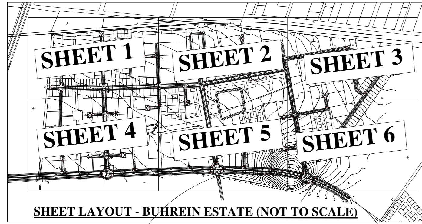
SHEET LAYOUT - BUH-REIN ESTATE (NOT TO SCALE) FOR LEGEND & NOTES - REFER TO SHEET 6
